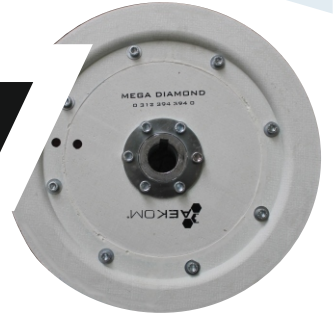
Aluminium or Composite Wheel for Quarry Machines. 300 mm - 500 mm - 600 mm - 700 mm - 800 mm - 1000 mm Diameter
